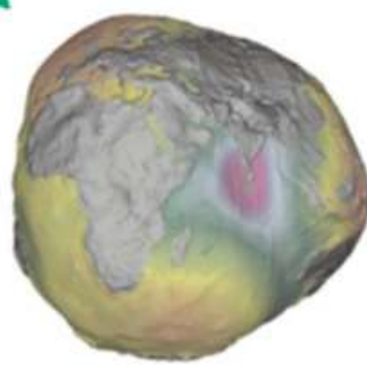
The Geoid
