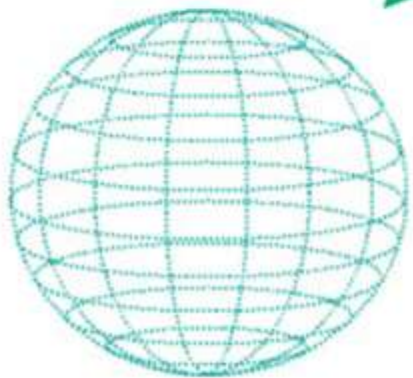
The ellipsoid
