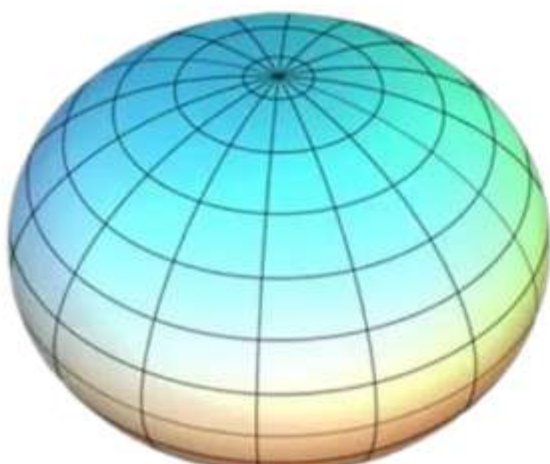
The ellipsoid
